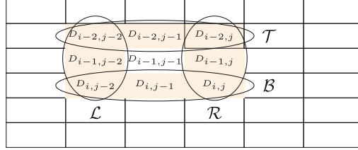
Fig. 2. Block of size 3
