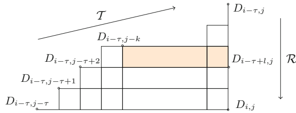
Fig. 3. Grid of size (\tau + 1) block
