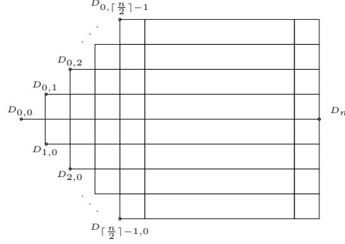
Fig. 4. Grid of (n + 1) -block
